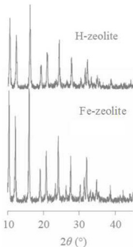
Figure 5. XRD patterns of H-zeolite and Fe-zeolite
