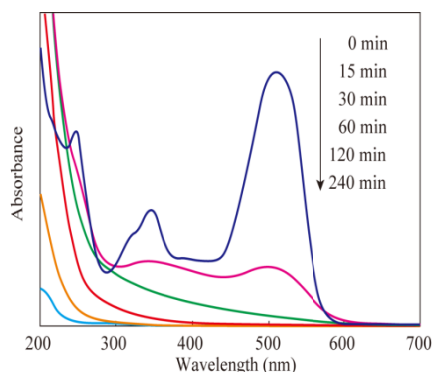
Figure 10 UV spectral changes with time.
