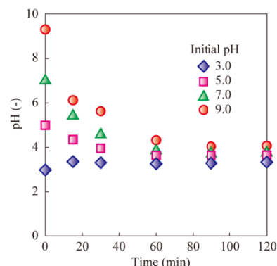
Figure 13. Changes in pH with time
