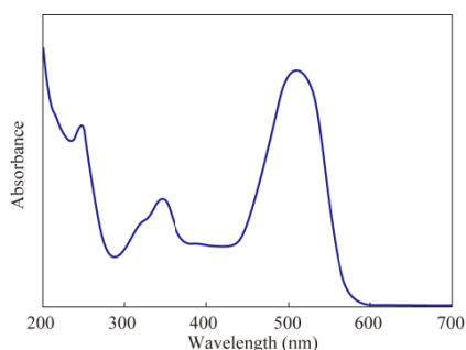
Figure 4. Absorption spectrum of Acid Red 88
